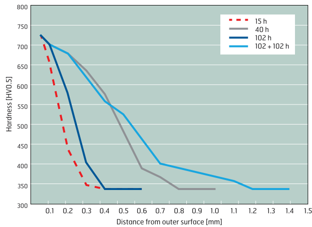
Gas nitriding of Toolox 33
